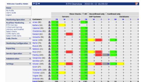
RealTime Monitoring Overview
